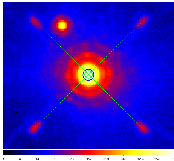
Figure 45 Non coronagraphic image of a star (happening to have a binary companion) in broad-band H with Irdi, after applying a waffle pattern to the DM for calibration purposes. The green thick circle indicates the intersection of the green lines, while the blue thick circle indicates the star position (Gaussian fit). Both agree within 2.5mas.
