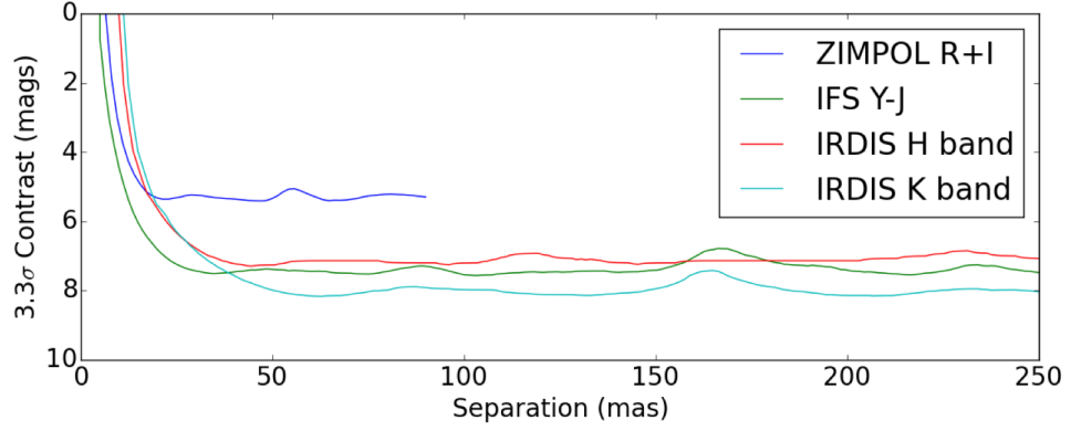
Figure 25: SAM_7H contrast limits for the detection of companions in various bands from the test data (July 2015). Each dataset consisted of approximately 1 hr in execution time, including time for observations of calibrator stars. This was obtained on the F6 star HD142527 with R=8.3 , J=6.5 , H=5.7 , K=4.98 with a seeing \sim 0.6\text{--}0.8'' . HIP113246 and HD169319 were used as calibrator stars (Cheetham et al., in prep.).
